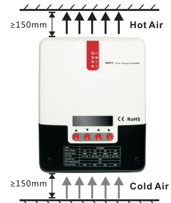
Figure 2-1 Installation and Heat Dissipation
