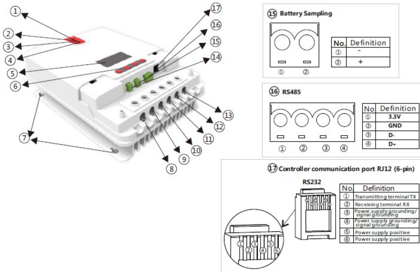
Fig. 1-1 Product appearance and interfaces
